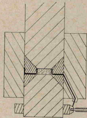
FIG. 3. High pressure ring, pellet, and sample geometry.
