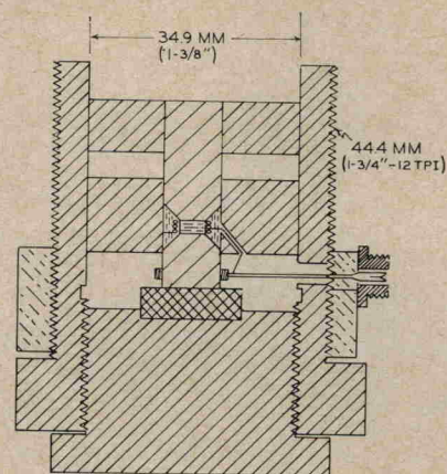
FIG. 2. High pressure NMR cell.
