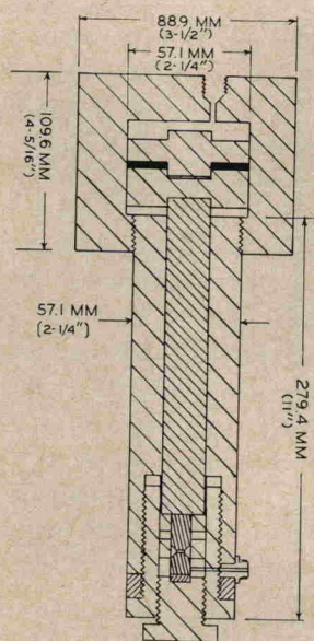
FIG. 1. High pressure NMR system.
